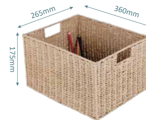
B85750 Storage Basket Medium Product Size: 360 x 265 x 175mm 14.2x10.4x6.9inches Package Size: 59x28x37.5cm 23.2x11x14.8inches QTY/CTN: 4pcs
