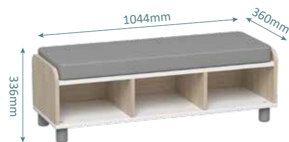
846067 Pisa Wooden Storage Seat Product Size: 1044x360x336mm 41.1x14.2x13.2inches Package Size: 112.5x40x20cm/102.5x73.5x3cm 44.3x15.7x7.9/40.4x28.9x1.2inches QTY/CTN: 1pc
