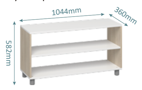
846027 Palermo Low 2 Layer Open Wood Shelf Product Size: 1044x360x582mm 41.1x14.2x22.9inches Package Size: 107.5x9.5x15.5cm 42.3x3.7x6.1inches QTY/CTN: 1pc
