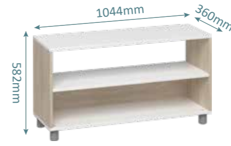
846028 Palermo Low 2 Layer Half Open Wood Shelf Product Size: 1044x360x582mm 41.1x14.2x22.9inches Package Size: 111x44x16.5cm 43.7x17.3x6.5inches QTY/CTN: 1pc
